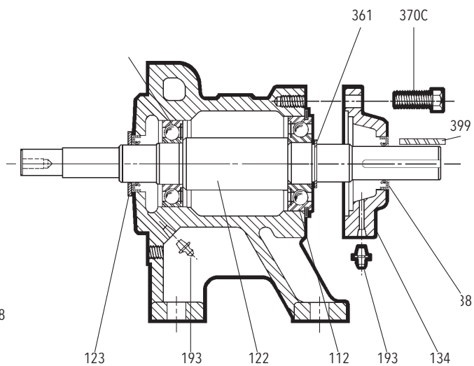
M-Group Power Frame
